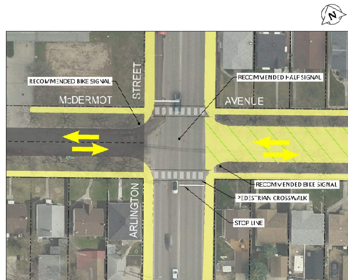
DETAIL A - MCDERMOT AVENUE AT ARLINGTON STREET
