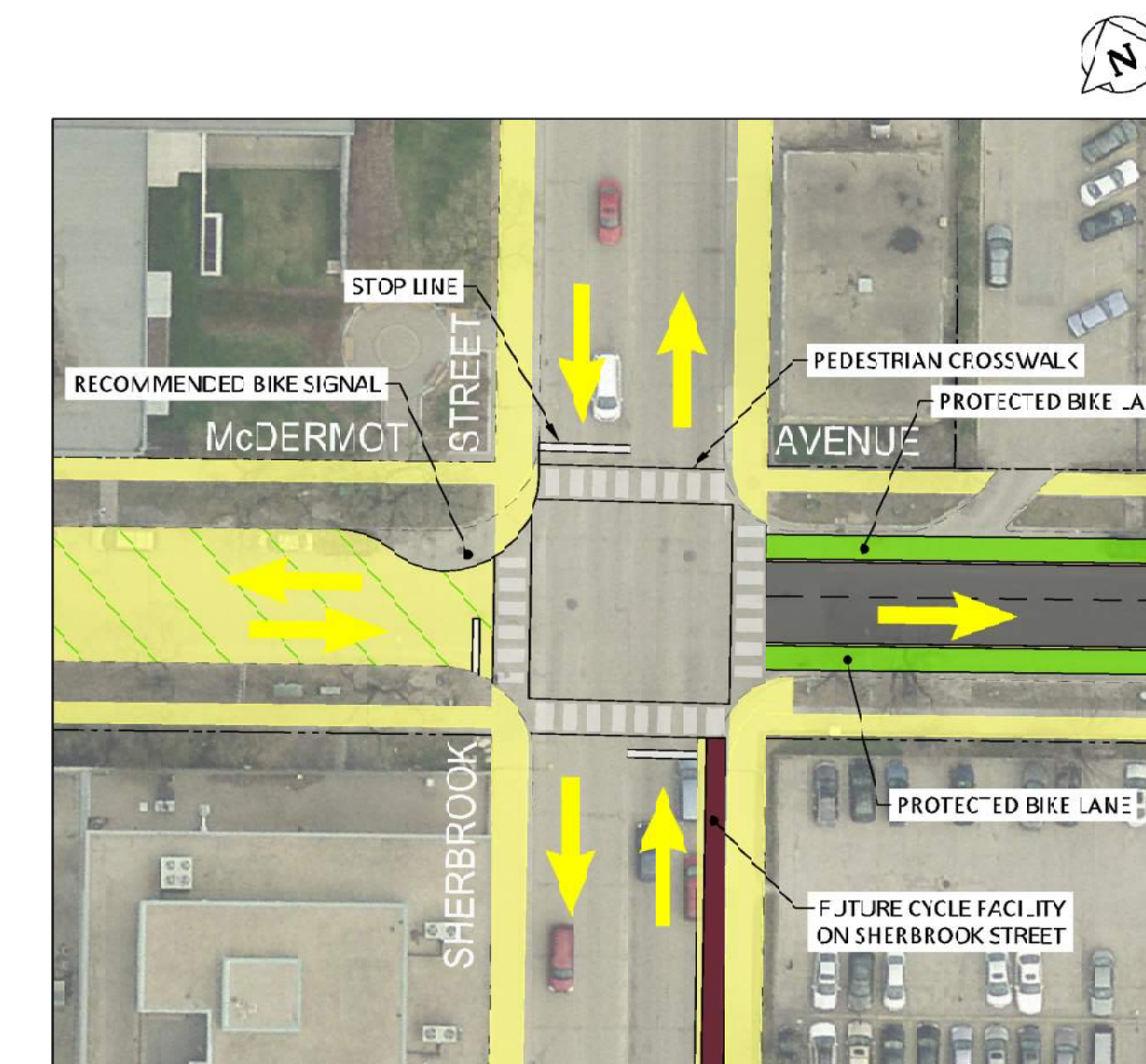
DETAIL B - MCDERMOT AVENUE AT SHERBROOK STREET
